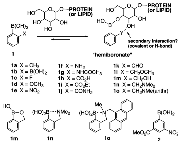
Figure 1. Ortho -substituted arylboronic acids tested for glycoside binding.
